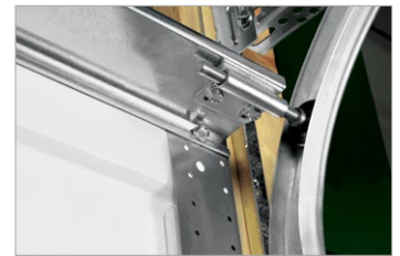
Top section roller slide attached to U-bar resists inward and outward force.
