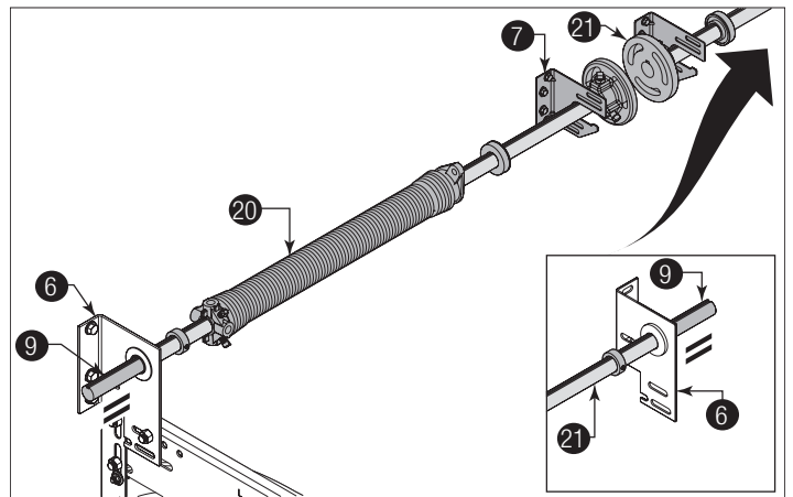
Figure 53, Left Side Shown
