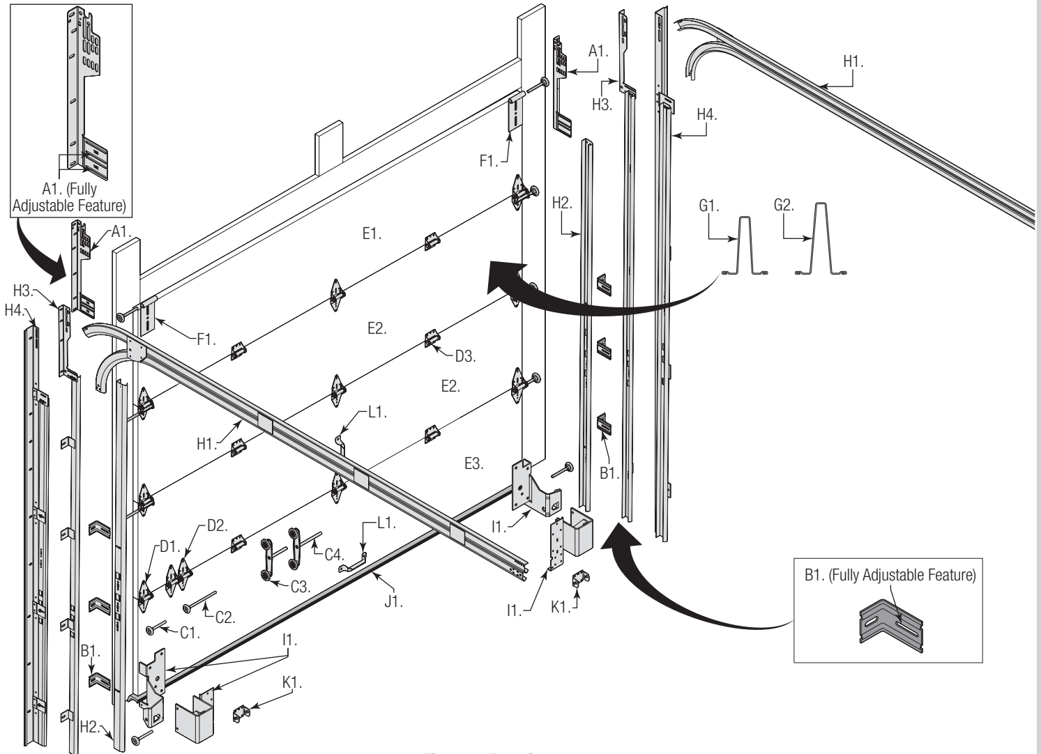
Figure 7 - Door Components
