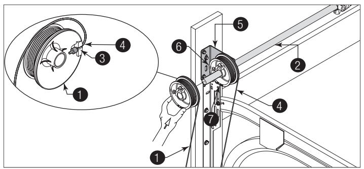
Figure 58, Left Side Shown
