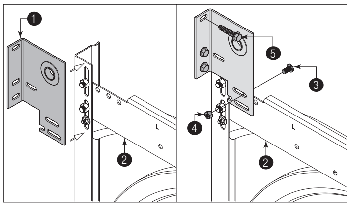
Figure 44, Left Side Shown (For M4. Bracket)
