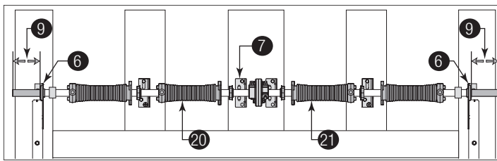
Figure 54, Left Side Shown
