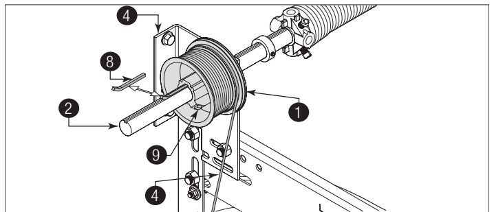
Figure 60, Left Side Shown
