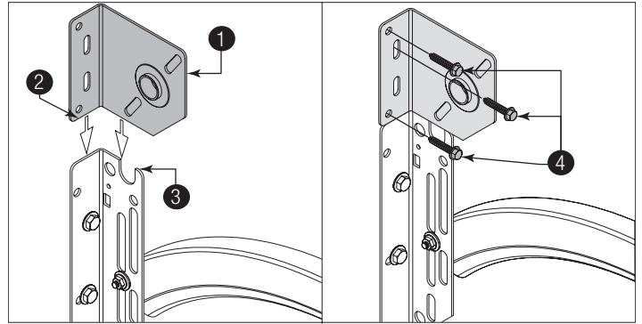
Figure 43, Left Side Shown (For M3. Bracket)
