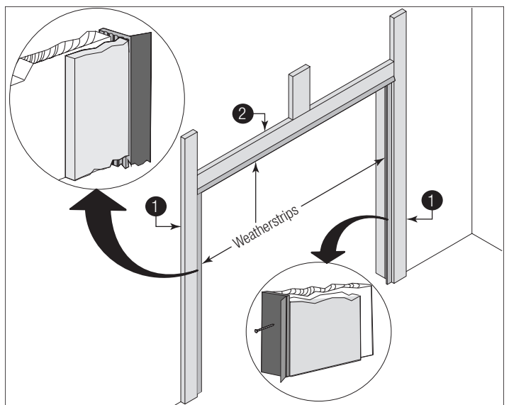
Figure 61, Weatherstrips
