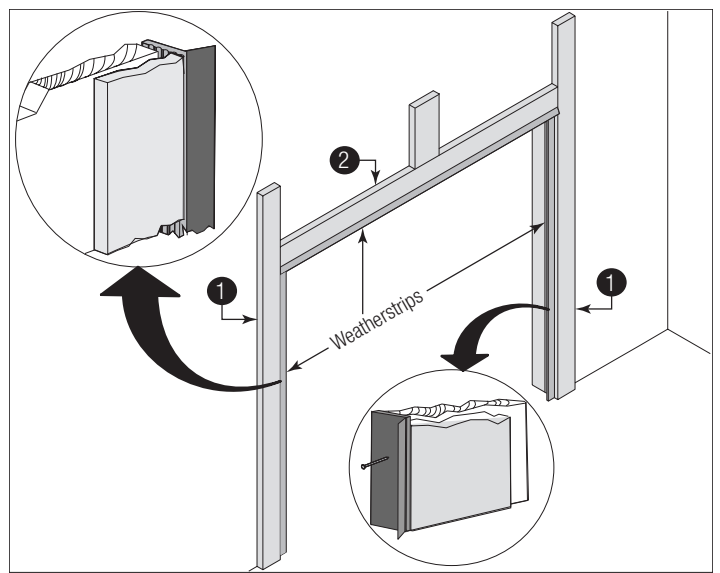
Figure 51, Weatherstrips
