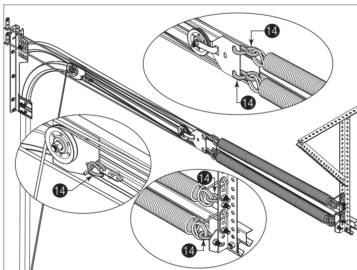
Figure 53, Left Side Shown
