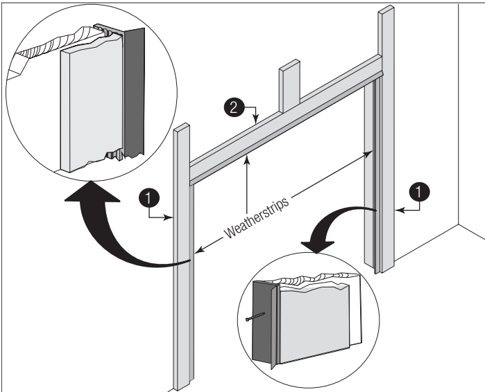
Figure 54, Weatherstrips
