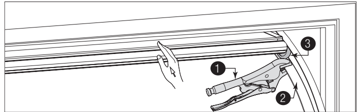
Figure 47, Outside Of The Door In The Open Position
