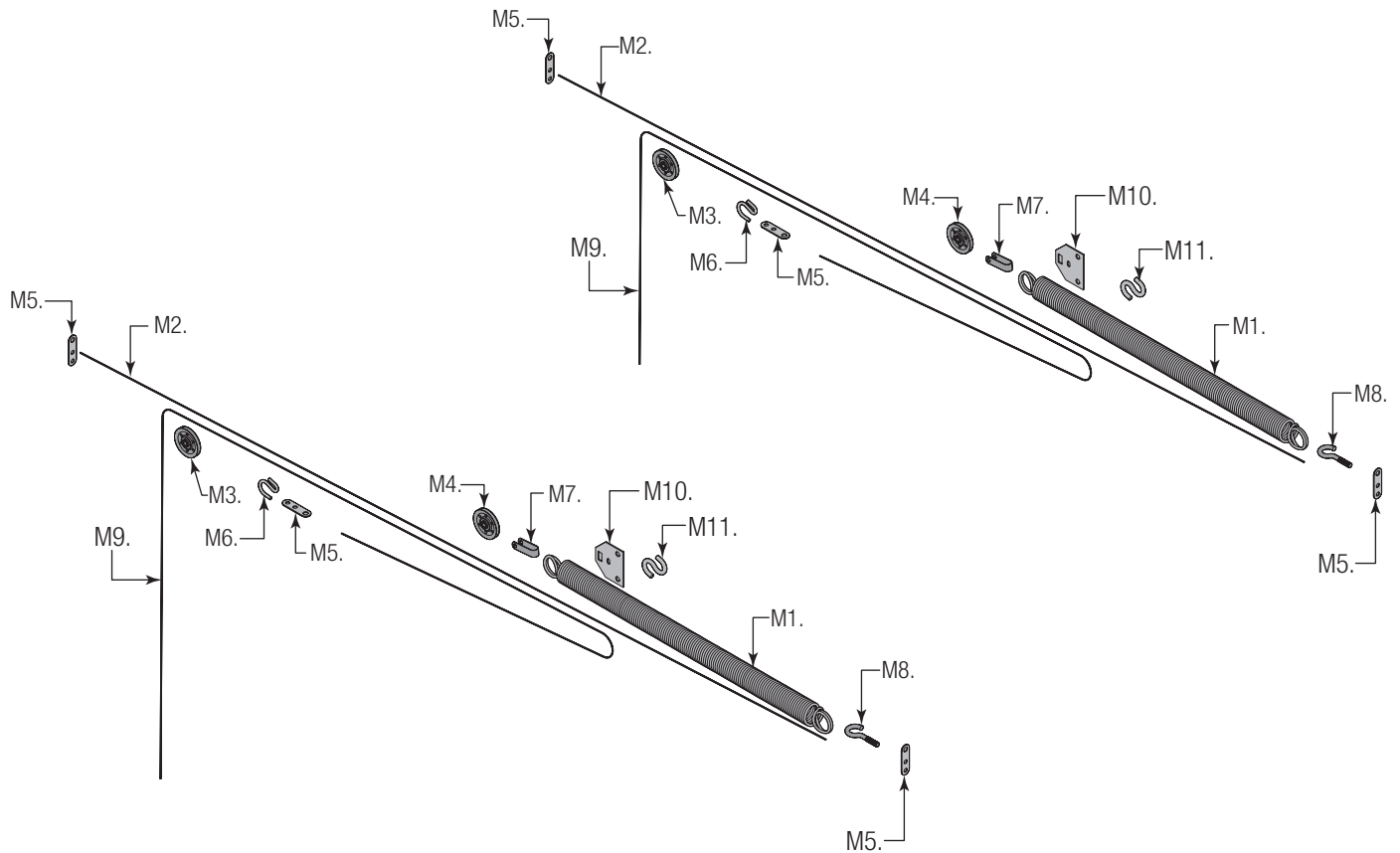
Figure 7 - Counterbalance Components
