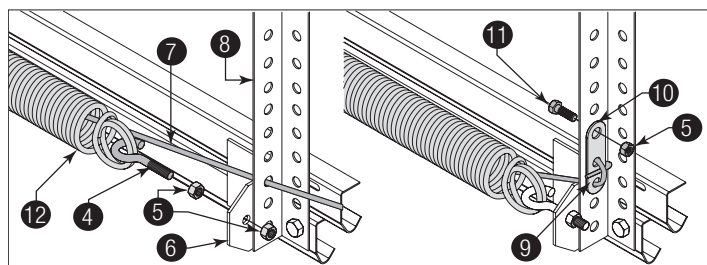
Figure 50, Left Side Shown
