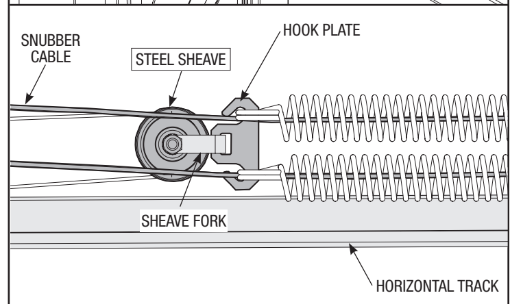
DOOR FEATURING 2 PAIRS OF EXTENSION SPRINGS
