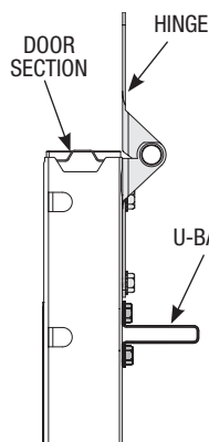
SIDE PROFILE
