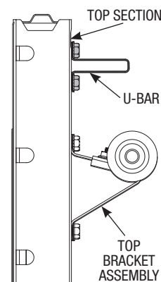
U-BAR PLACEMENT FOR TOP SECTION
