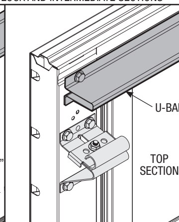
U-BAR PLACEMENT FOR TOP SECTION
