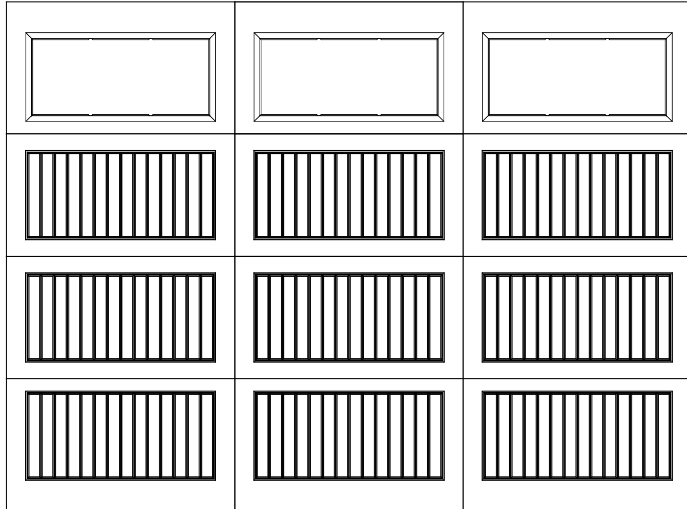
12 X 9 9800 SONOMA DESIGN 4 SECTION/3 PANEL PLAIN GLAZED SQUARE TOP SECTION SHOWN CONSISTS OF (2) 27.73" & (2) 25.73" SECTIONS
