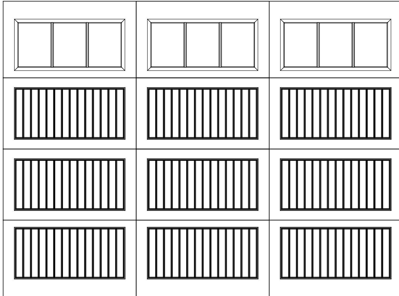
12 X 9 9800 SONOMA DESIGN 4 SECTION/3 PANEL 9 LITE SQUARE TOP SECTION SHOWN CONSISTS OF (2) 27.73" & (2) 25.73" SECTIONS
