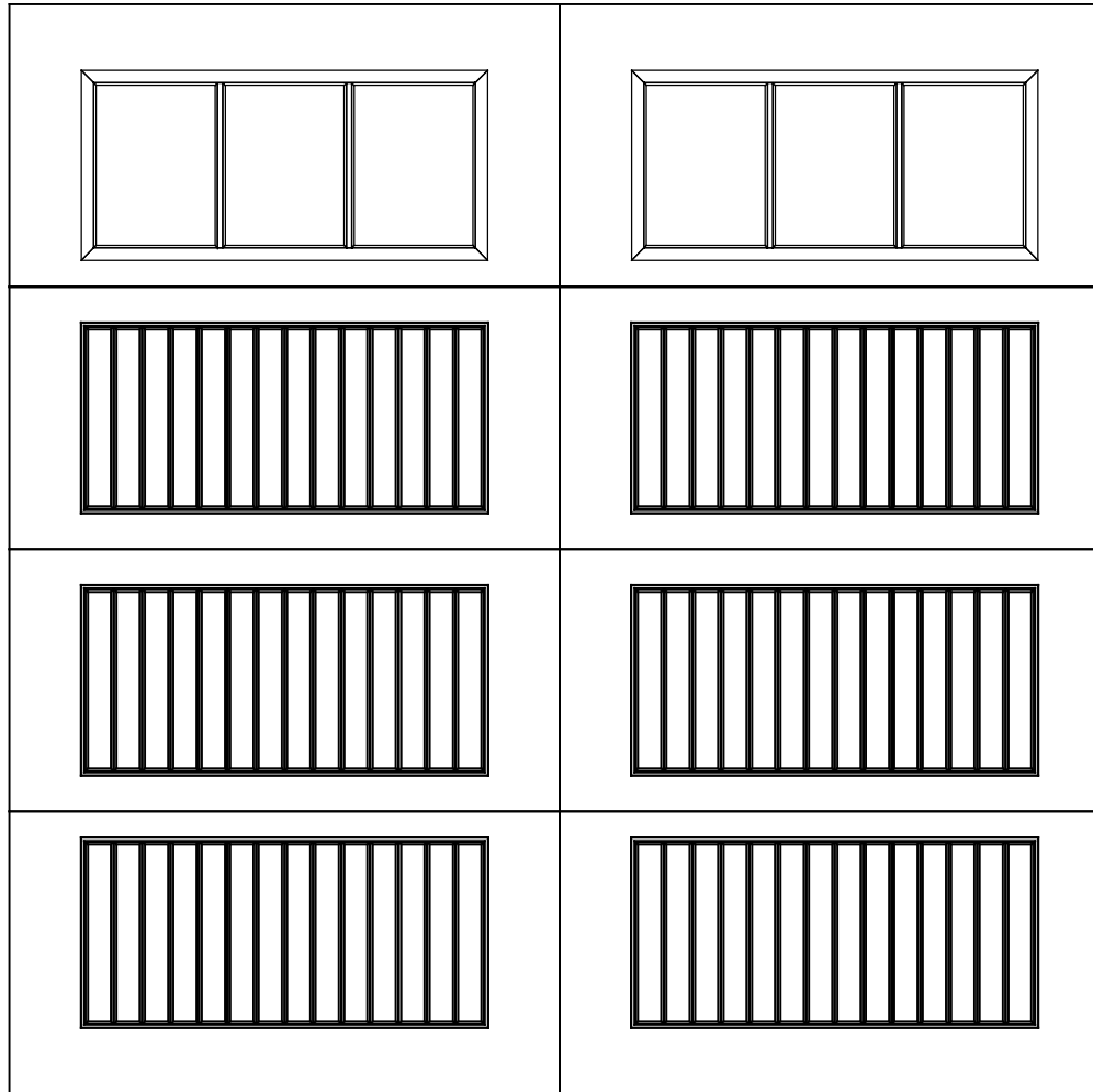
9 X 9 9800 SONOMA DESIGN 4 SECTION/2 PANEL 6 LITE SQUARE TOP SECTION SHOWN CONSISTS OF (2) 27.73" SECTIONS & (2) 25.73" SECTIONS
