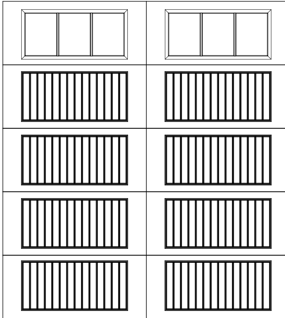
9' x 10' 9800 SONOMA 5 SECTION/2 PANEL 6 LITE SQUARE TOP SECTION SHOWN CONSISTS OF (5) 23.8" SECTIONS
