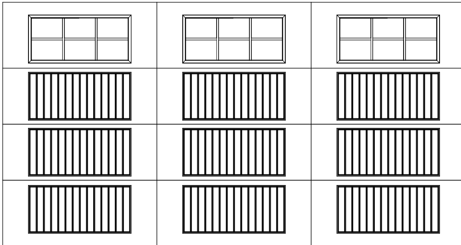
15' x 8' 9800 SONOMA 4 SECTIONS/3 PANELS 18 LITE SQUARE TOP SECTION SHOWN CONSISTS OF (2) 25.73" & (2) 21.88" SECTIONS
