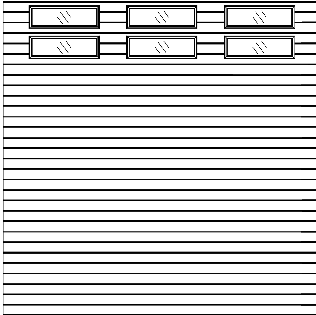
10x10 9800 HVG DESIGN HORIZONTAL GLAZED TOP SECTION CONSISTS OF (5) 23.80" SECTIONS
