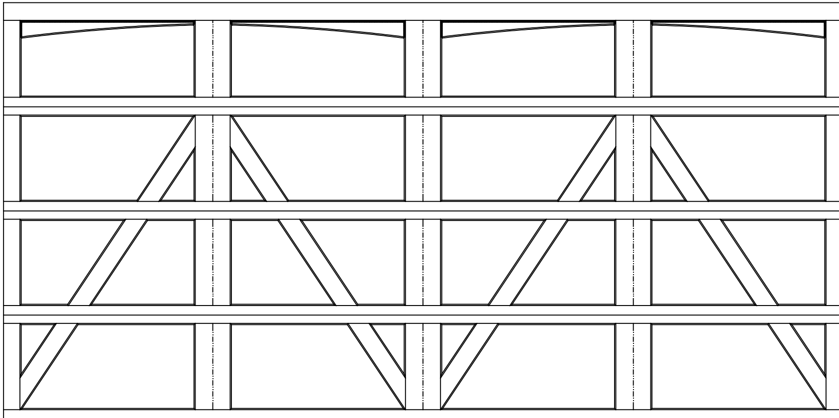
16'0" X 8'0" 9700 CHARLESTON DESIGN 4 SECTION/4 PANEL DOUBLE SOLID ARCHED TOP SECTION SHOWN (4) 23.8" SECTIONS
