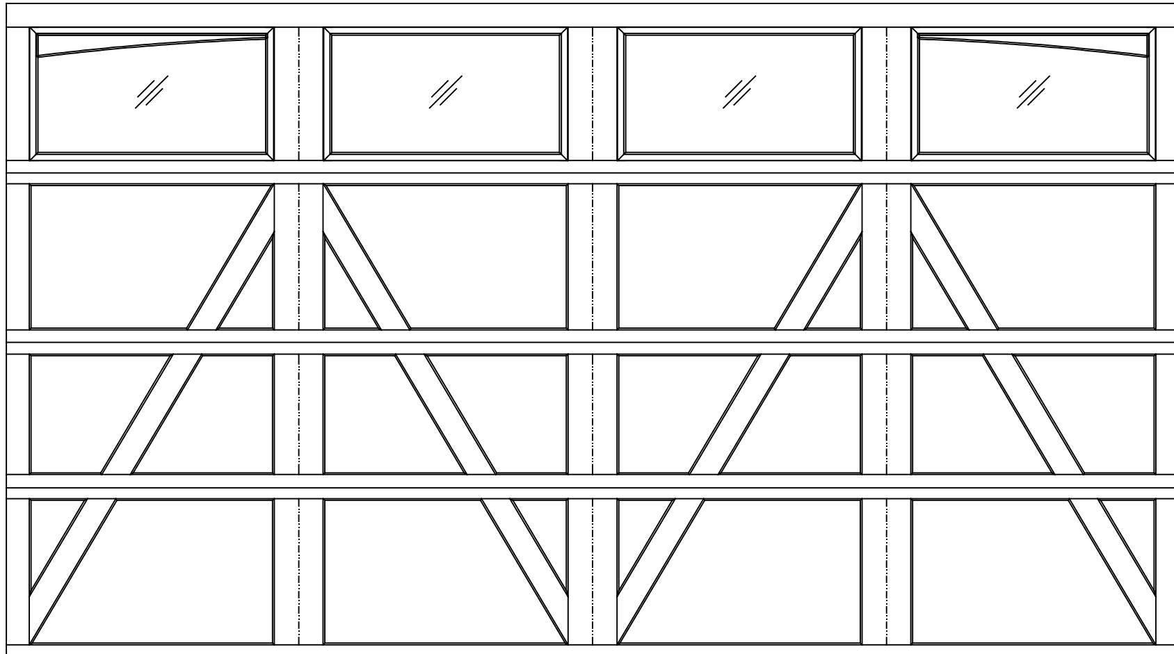
16'0" X 9'0" 9700 CHARLESTON DESIGN 4 SECTION/4 PANEL SINGLE PLAIN ARCHED TOP SECTION SHOWN (1) 23.8" & (3) 27.73" SECTIONS
