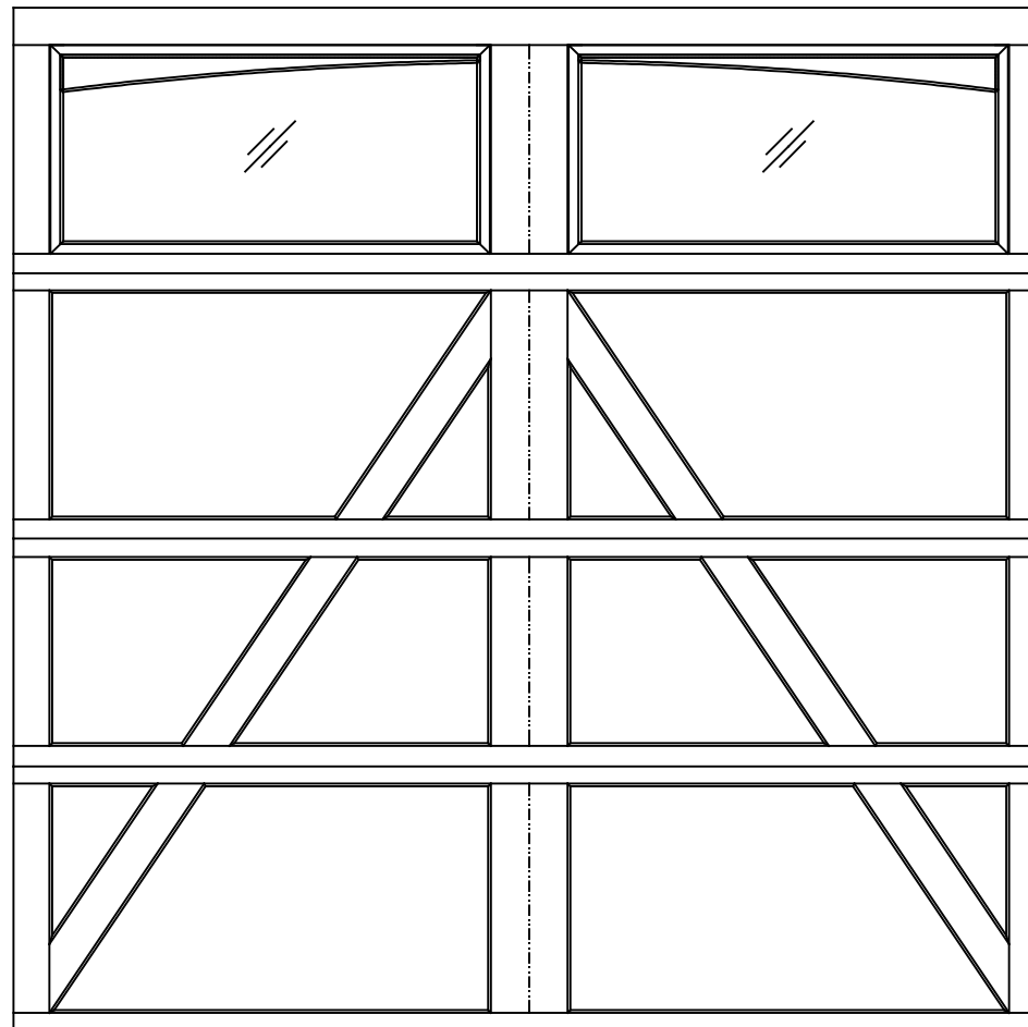
9'0" X 9'0" 9700 CHARLESTON DESIGN 4 SECTION/2 PANEL PLAIN ARCHED TOP SECTION SHOWN (1) 23.8" & (3) 27.73" SECTIONS
