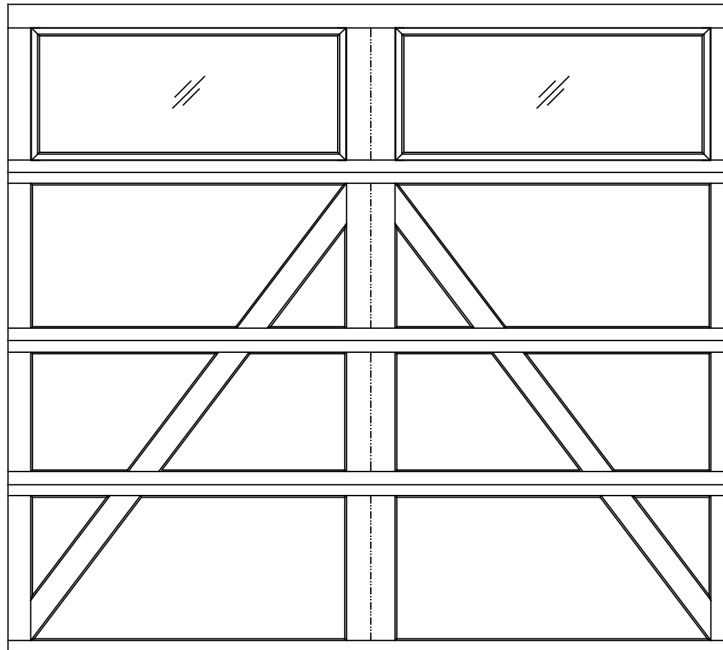
10'0" X 9'0" 9700 CHARLESTON DESIGN 4 SECTION/2 PANEL PLAIN TOP SECTION SHOWN (1) 23.8" & (3) 27.73" SECTIONS
