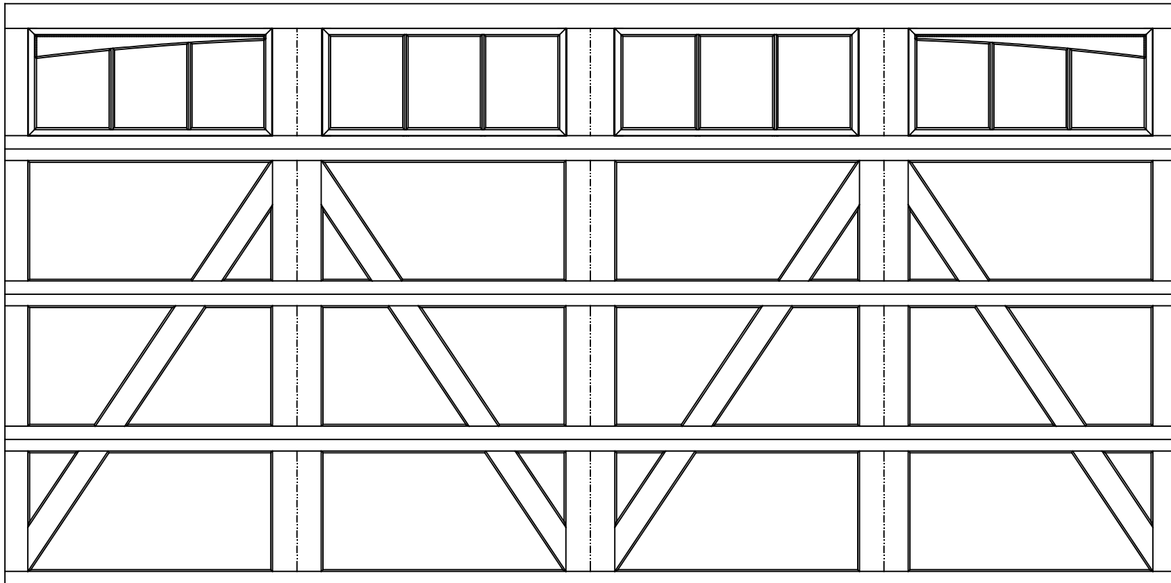
16'0" X 8'0" 9700 CHARLESTON DESIGN 4 SECTION/4 PANEL SINGLE 12 LITE ARCHED TOP SECTION SHOWN (4) 23.8" SECTIONS
