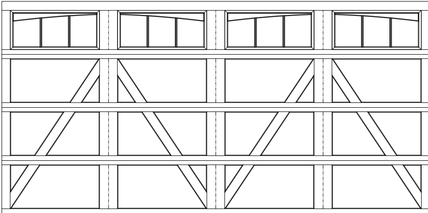
16'0" X 8'0" 9700 CHARLESTON DESIGN 4 SECTION/4 PANEL DOUBLE 12 LITE ARCHED TOP SECTION SHOWN (4) 23.8" SECTIONS
