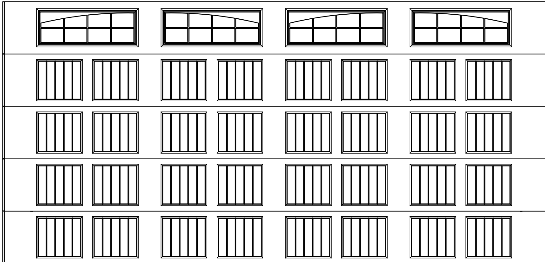
18' X 8'9" 9100/9605 SONOMA DESIGN 5 SECTION/8 PANEL DOUBLE ARCH STOCKTON III TOP SECTION SHOWN CONSISTS OF (5) 20.8" SECTIONS
