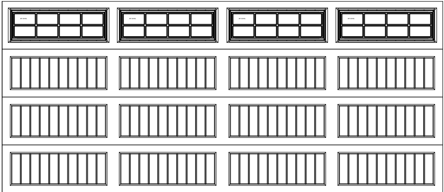
16 X 8 9100/9605 SONOMA RANCH 4 SECTIONS/4 PANELS STOCKTON IV 8LITE TOP SECTION SHOWN CONSISTS OF (4) 23.8" SECTIONS
