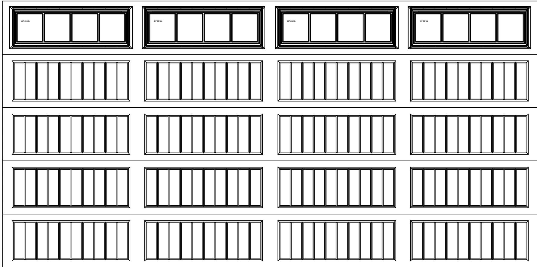
16 X 8 9100/9605 SONOMA RANCH 5 SECTIONS/4 PANELS STOCKBRIDGE IV 4LITE TOP SECTION SHOWN CONSISTS OF (5) 19.1" SECTIONS
