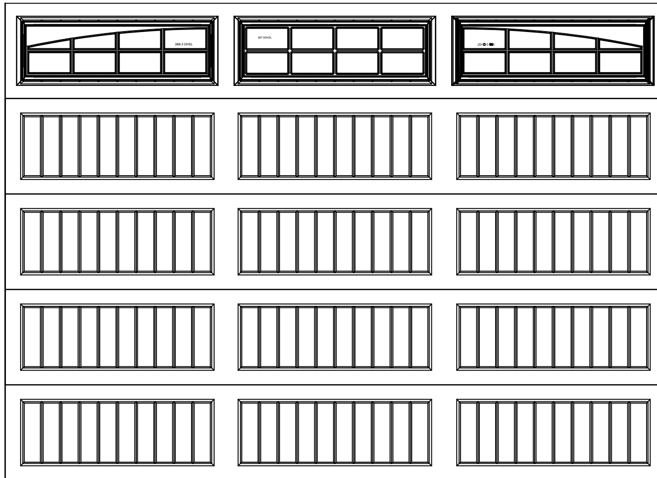
12 X 9 9100/9605 SONOMA RANCH 5 SECTIONS/4 PANELS ARCH STOCKTON IV TOP SECTION SHOWN CONSISTS OF (4) 20.8" & (1) 23.8" SECTIONS
