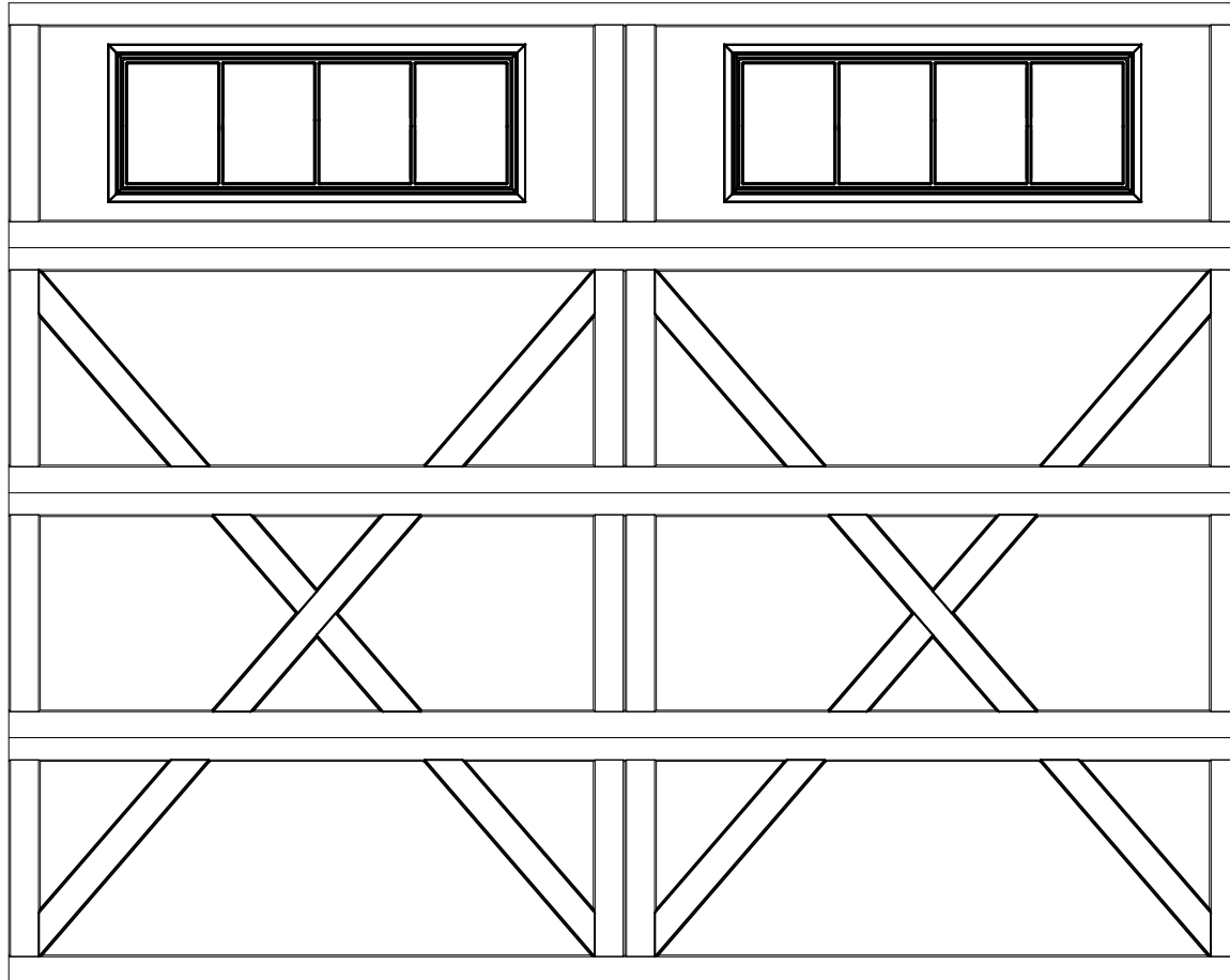
10'0" X 8'0" 9405 LEXINGTON 4 SECTION / 2 PANEL STOCKBRIDGE TOP SECTION SHOWN CONSISTS OF (4) 23.8" SECTIONS
