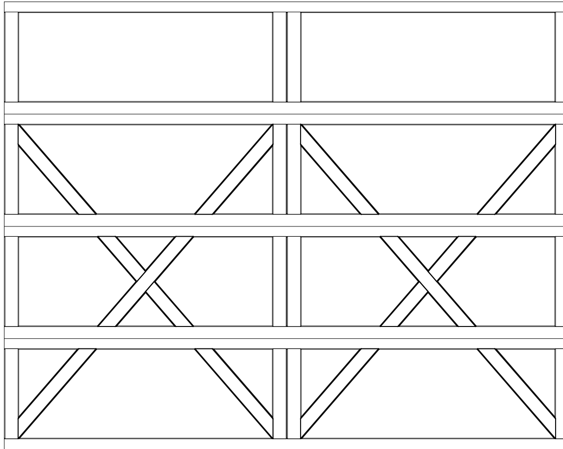
10'0" X 8'0" 9405 LEXINGTON 4 SECTION / 2 PANEL SOLID TOP SECTION SHOWN CONSISTS OF (4) 23.8" SECTIONS
