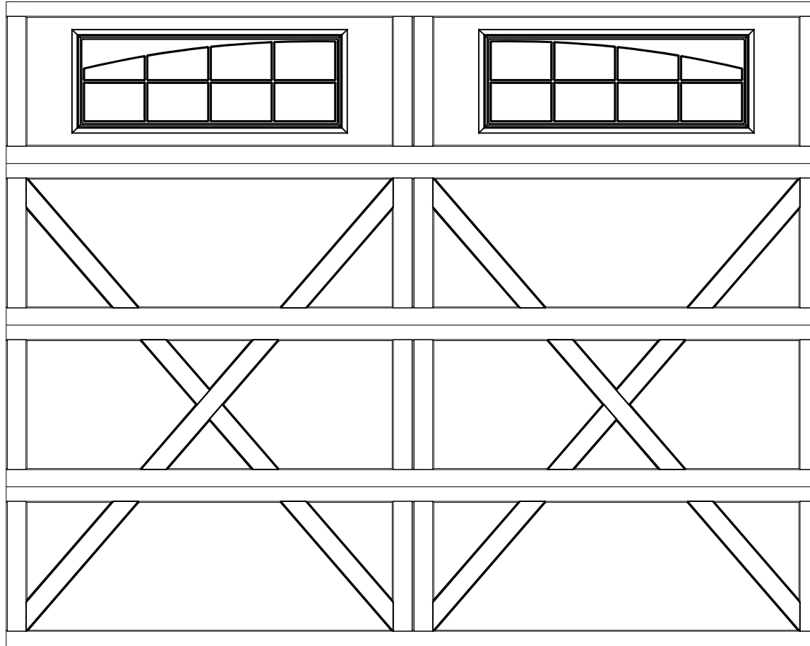
10'0" X 8'0" 9405 LEXINGTON 4 SECTION / 2 PANEL ARCH STOCKTON III TOP SECTION SHOWN CONSISTS OF (4) 23.8" SECTIONS
