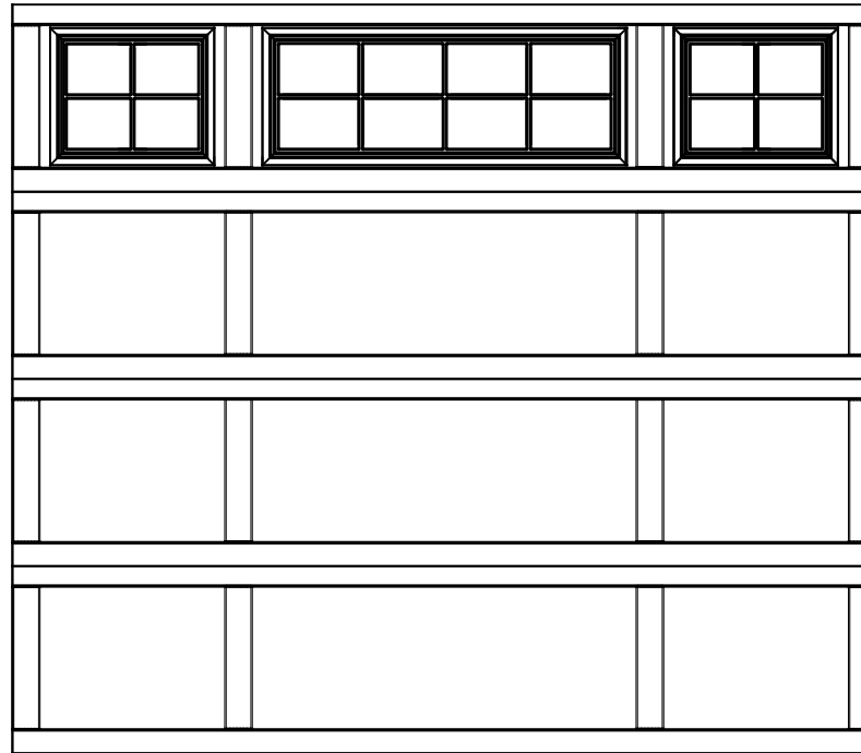
8x7 9405 HAMPTON 4 SECTION/3 PANEL STOCKTON III TOP SECTION SHOWN CONSISTS OF (4) 20.8" SECTIONS
