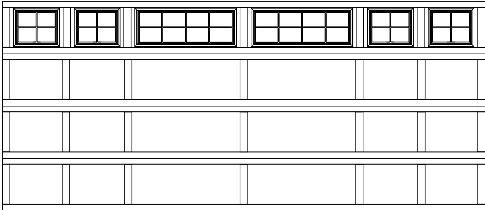
16x8 9405 HAMPTON 4 SECTION/6 PANEL STOCKTON TOP SECTION SHOWN CONSISTS OF (4) 23.8" SECTIONS
