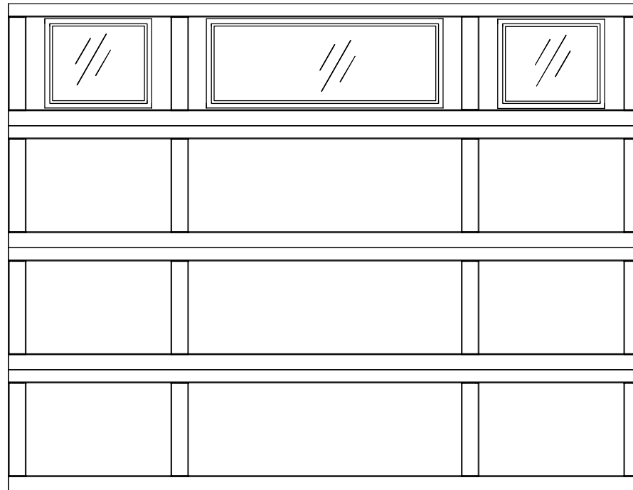
9x7 9405 HAMPTON 4 SECTION/3 PANEL GLAZED TOP SECTION SHOWN CONSISTS OF (4) 20.8" SECTIONS
