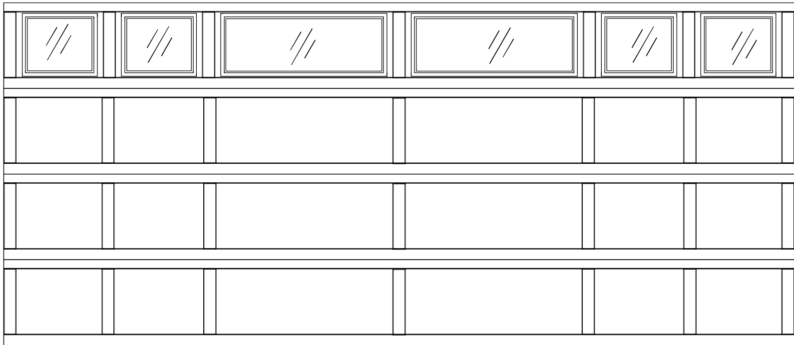
16x7 9405 HAMPTON 4 SECTION/6 PANEL GLAZED TOP SECTION SHOWN CONSISTS OF (4) 20.8" SECTIONS
