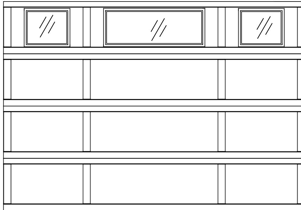
10x8 9405 HAMPTON 4 SECTION/3 PANEL GLAZED TOP SECTION SHOWN CONSISTS OF (4) 23.8" SECTIONS
