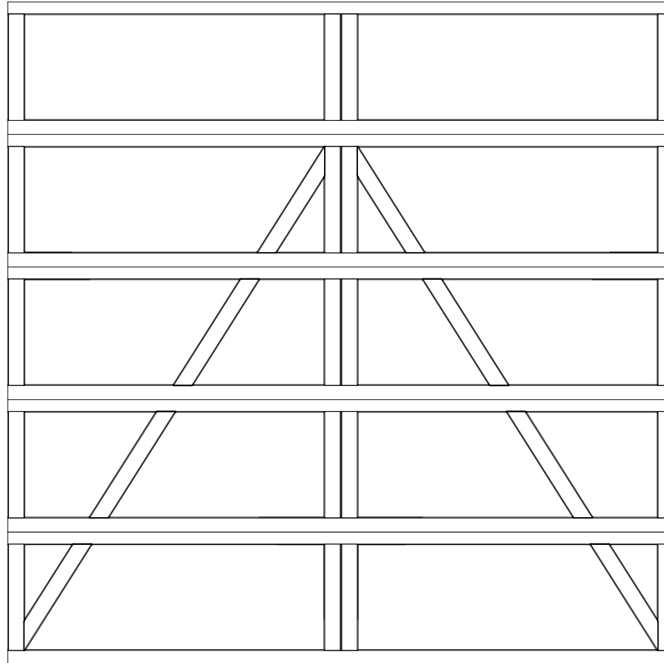
10'0" X 10'0" 9405 CHARLESTON 5 SECTION / 2 PANEL SOLID TOP SECTION SHOWN CONSISTS OF (5) 23.8" SECTIONS
