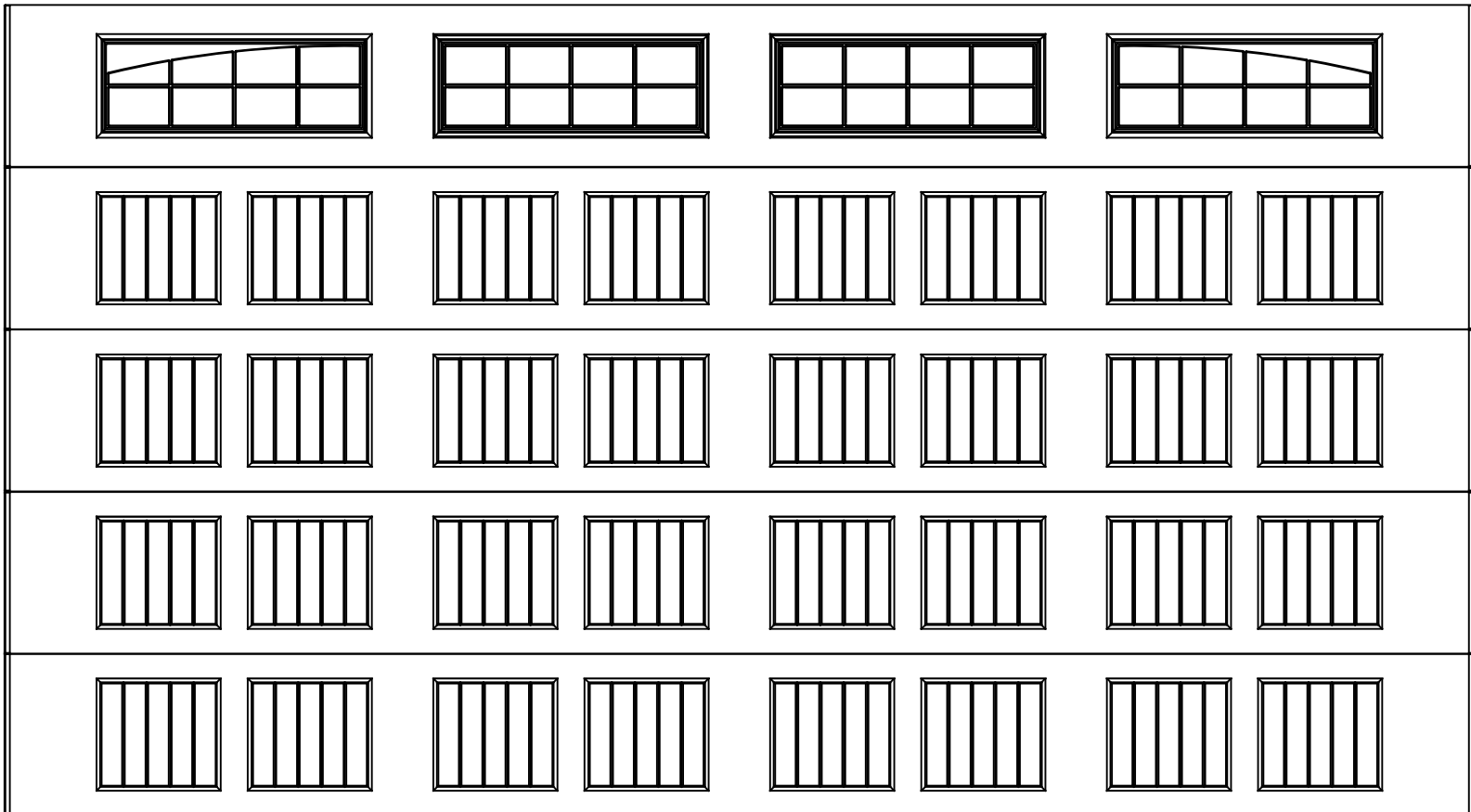
18 X 10 9605 SONOMA DESIGN 5 SECTION/8 PANEL ARCH STOCKTON III TOP SECTION SHOWN CONSISTS OF (5) 23.8" SECTIONS
