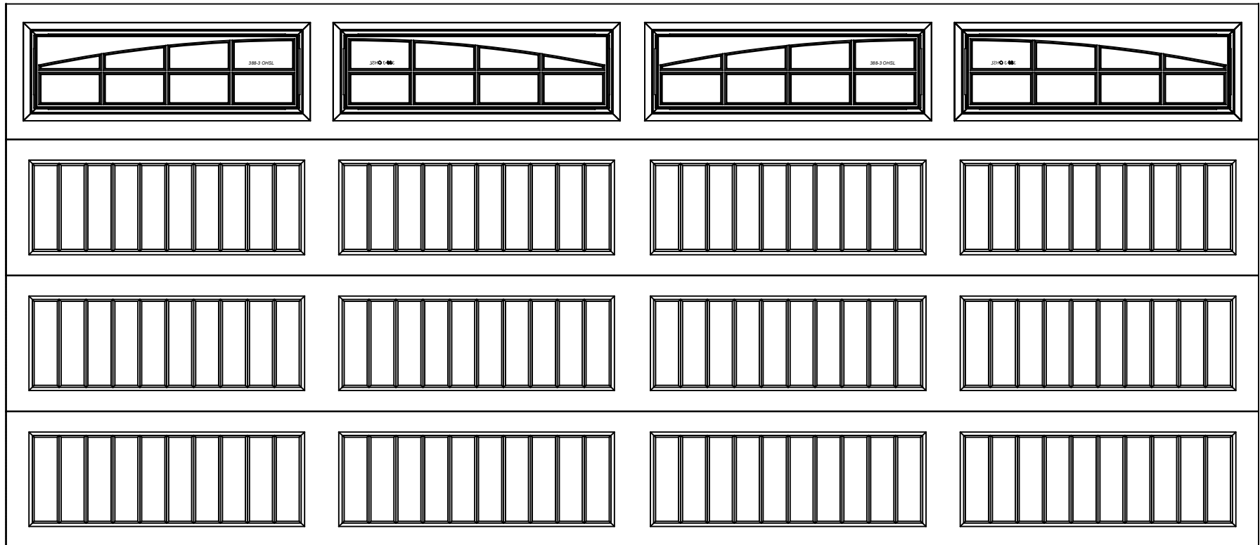
16 X 8 9605 SONOMA RANCH 4 SECTIONS/4 PANELS DOUBLE ARCH STOCKTON IV TOP SECTION SHOWN CONSISTS OF (4) 23.8" SECTIONS
