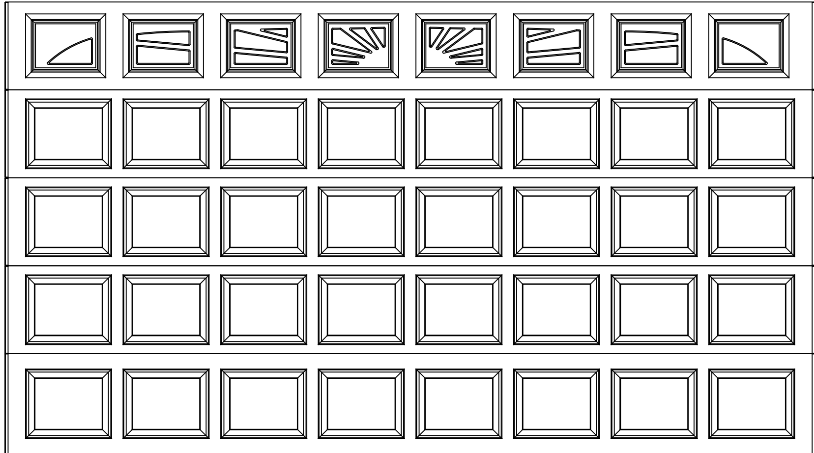
16 X 9 9100/9605 CRP DESIGN 5 SECTION/8 PANEL SINGLE WILLIAMSBURG I TOP SECTION SHOWN CONSISTS OF (4) 20.8" & (1) 23.8" SECTIONS
