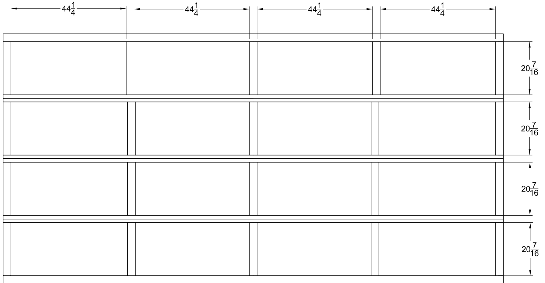
16'-0"x8'-0" 8800 4 SECTION/4 PANEL
