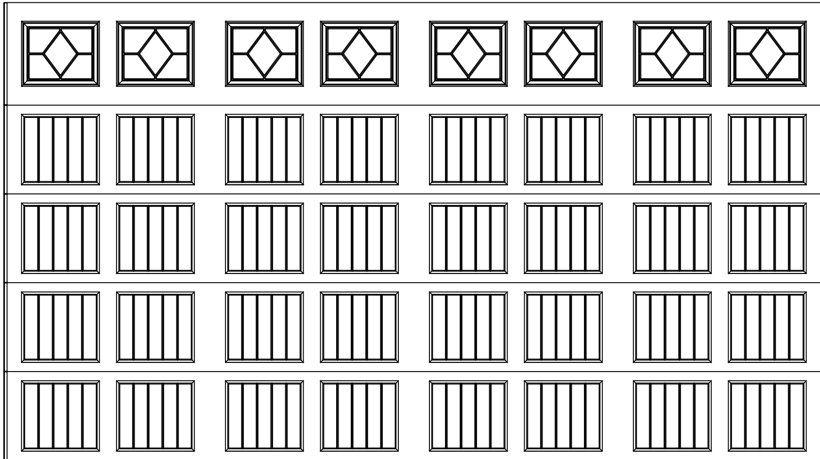
16'0" X 9'0" 8300/8500 SONOMA DESIGN 5 SECTION / 8 PANEL WATERTON I TOP SECTION (4) 20.8" & (1) 24.0" SECTIONS
