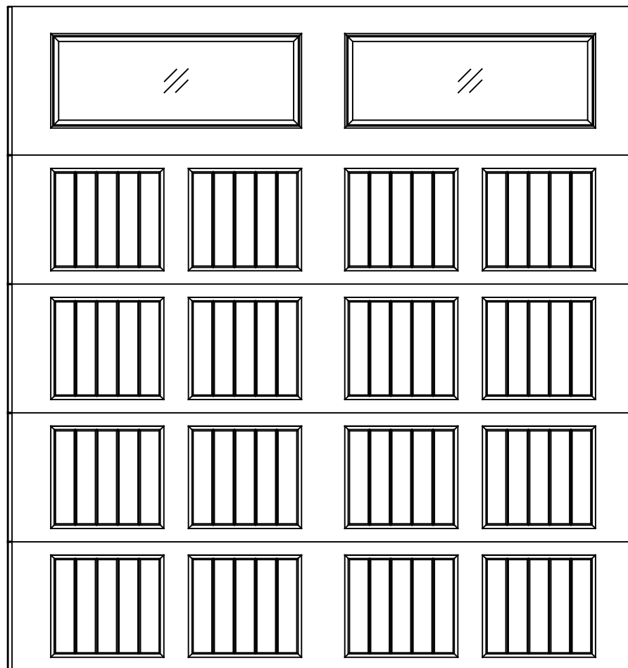
8'6" X 9'0" 8300/8500 SONOMA DESIGN 5 SECTION/ 4 PANEL STYLELINE III TOP SECTION (4) 20.8" & (1) 24.0" SECTIONS
