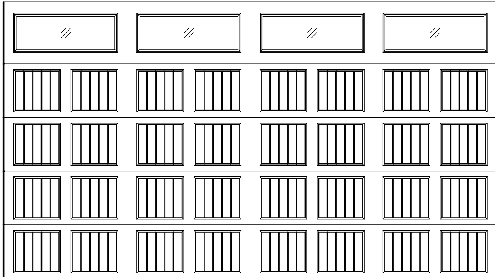
16'0" X 9'0" 8300/8500 SONOMA DESIGN 4 SECTION/ 8 PANEL STYLELINE III TOP SECTION (4) 20.8" & (1) 24.0" SECTIONS
