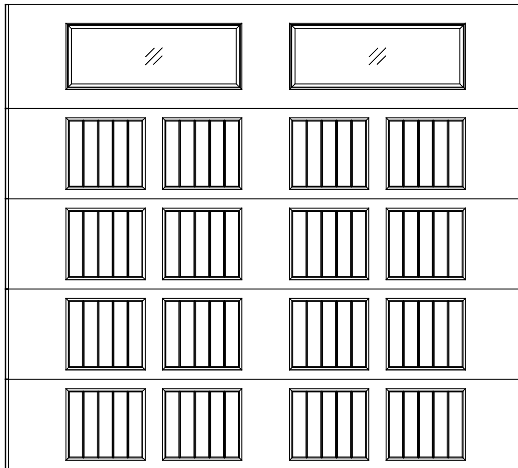
10'0" X 9'0" 8300/8500 SONOMA DESIGN 5 SECTION/ 4 PANEL STYLELINE III TOP SECTION (4) 20.8" & (1) 24.0" SECTIONS
