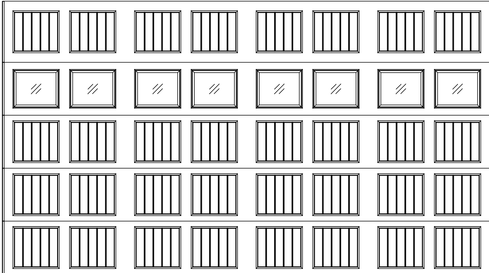
16'0" X 9'0" 8300/8500 SONOMA DESIGN 5 SECTION/ 8 PANEL STYLELINE I INTERMEDIATE 4 SECTION SHOWN (4) 20.8" & (1) 24.0" SECTIONS
