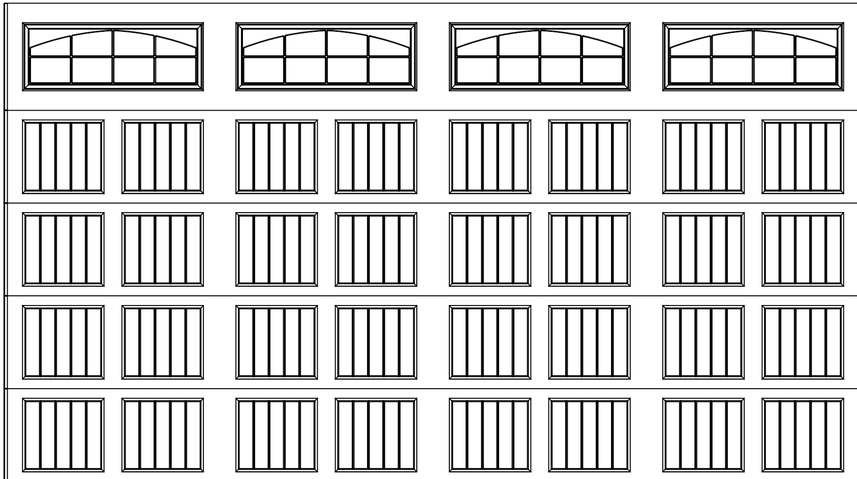
16'0" X 9'0" 8300/8500 SONOMA DESIGN 5 SECTION/ 8 PANEL CASCADE III TOP SECTION (4) 20.8" & (1) 24.0" SECTIONS
