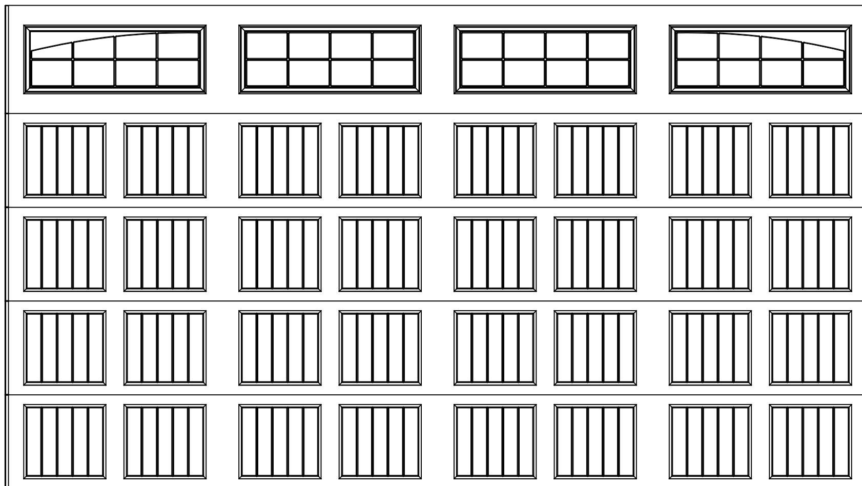
16'0" X 9'0" 8300/8500 SONOMA DESIGN 5 SECTION / 8 PANEL SINGLE ARCHED STOCKTON III TOP SECTION (4) 20.8" & (1) 24.0" SECTIONS
