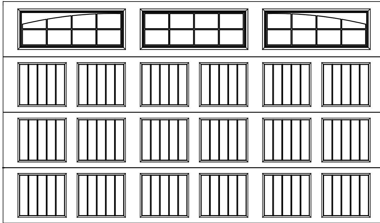
12'x7' 8300/8500 SONOMA ARCHED STOCKTON III TOP SECTION (4) 20.8" SECTIONS
