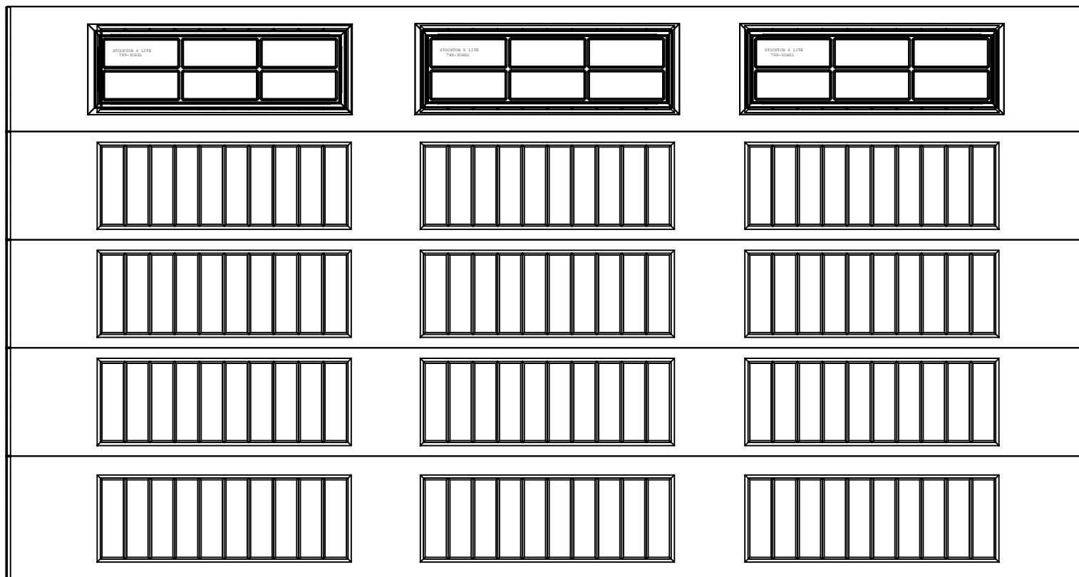
15'x8' 8300 SONOMA RANCH 4 SECTION/3 PANEL STOCKTON IV 6LITE TOP SECTION SHOWN CONSISTS OF (2) 20.8" & (3) 18" SECTIONS
