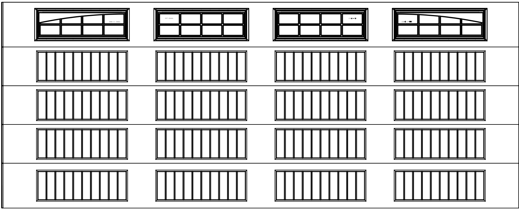
20'x8' 8300 SONOMA RANCH 5 SECTION/4 PANEL SINGLE ARCHSTOCKTON IV TOP SECTION SHOWN CONSISTS OF (2) 20.8" & (3) 18" SECTIONS
