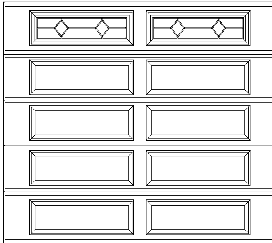
9'0" X 8'0" 8300/8500 ERP DESIGN 5 SECTION/ 2 PANEL WATERTON II TOP SECTION SHOWN (3) 18" & (2) 20.8" SECTIONS
