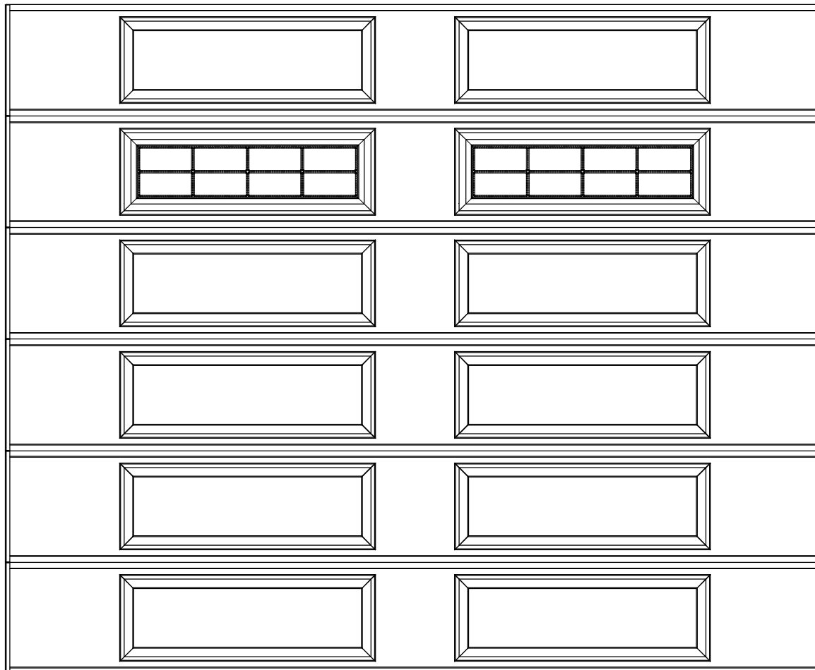
11'0" X 9'0" 8300/8500 ERP DESIGN 6 SECTION / 2 PANEL STOCKTON II INTERMEDIATE 5 SECTION SHOWN (6) 18" SECTIONS
