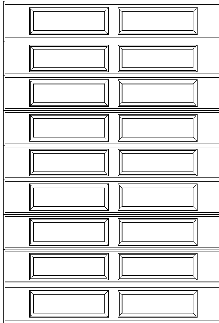
9'6" X 14'0" 8300/8500 ERP DESIGN 8 SECTION / 2 PANEL SOLID TOP SECTION (7) 18" & (2) 20.8" SECTIONS
