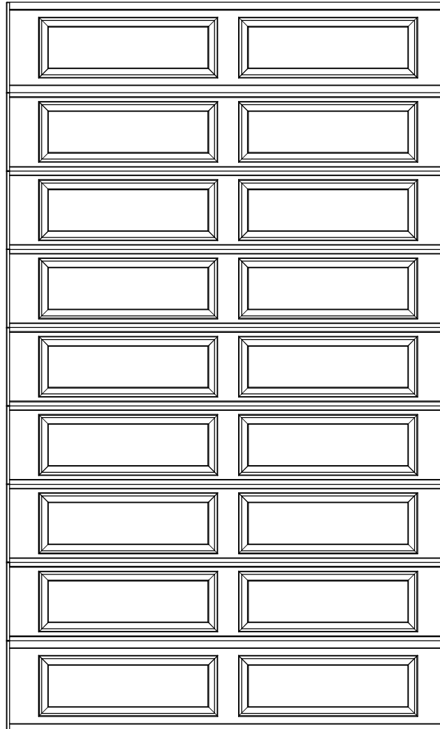
8'6" X 14'0" 8300/8500 ERP DESIGN 8 SECTION / 2 PANEL SOLID TOP SECTION (7) 18" & (2) 20.8" SECTIONS
