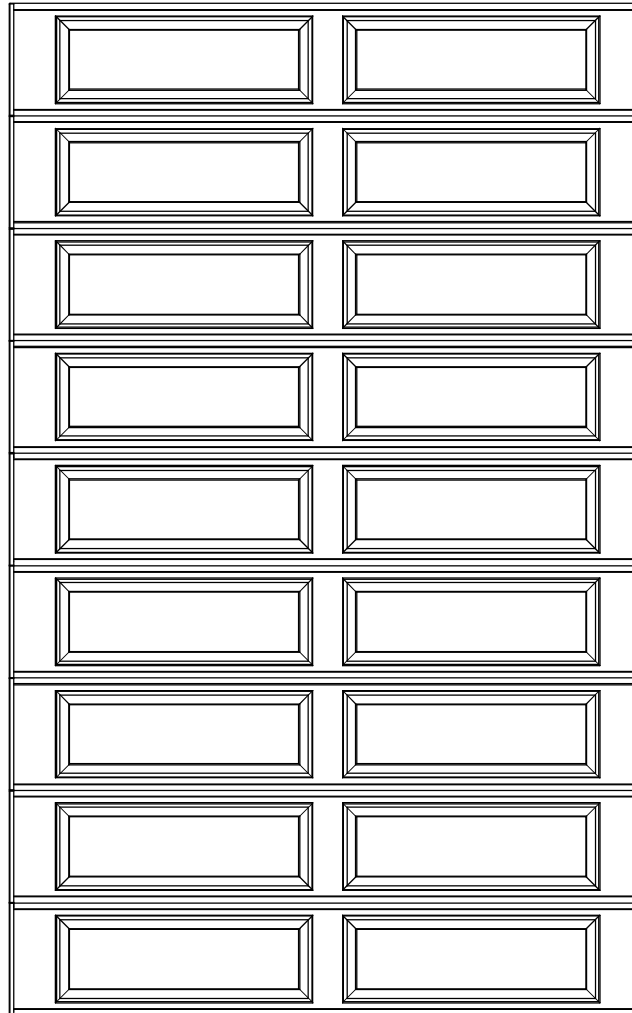
8'6" X 13'6" 8300/8500 ERP DESIGN 8 SECTION / 2 PANEL SOLID TOP SECTION (9) 18" SECTIONS
